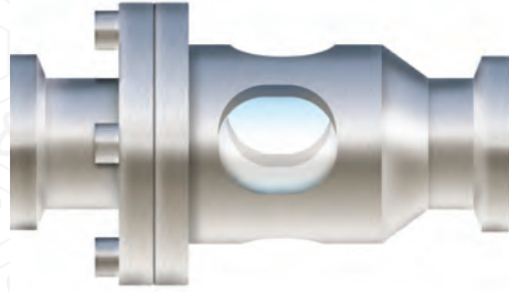
Bolted Sight Gauge
